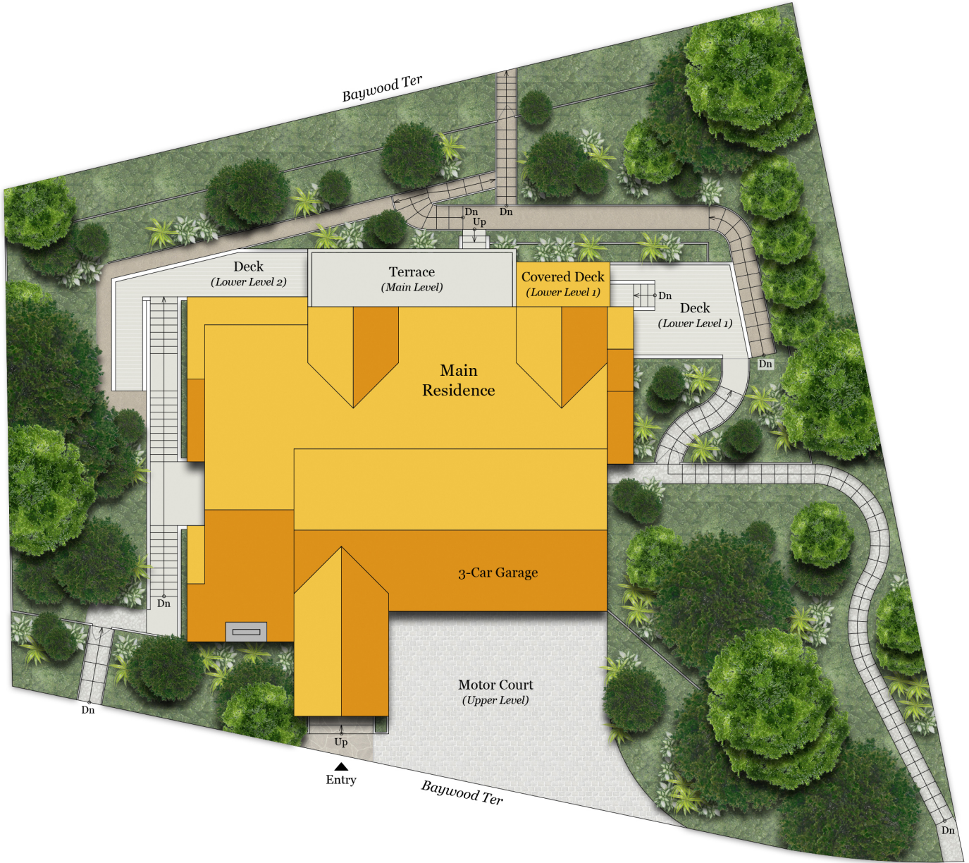
SITE PLAN
