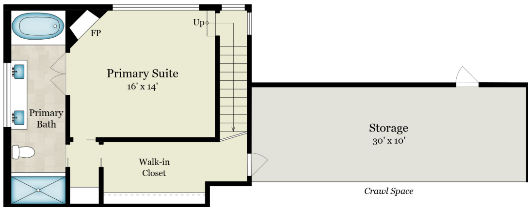
LOWER LEVEL
