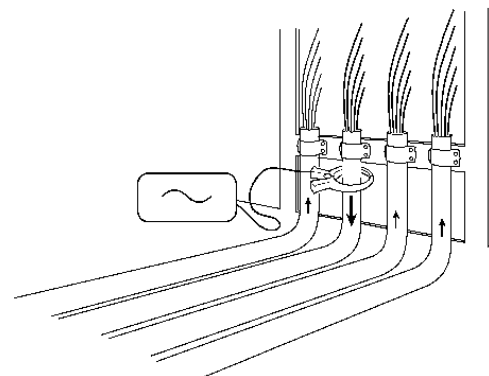
Figures 9.5 – 9.6: Connecting transmitter clamps
