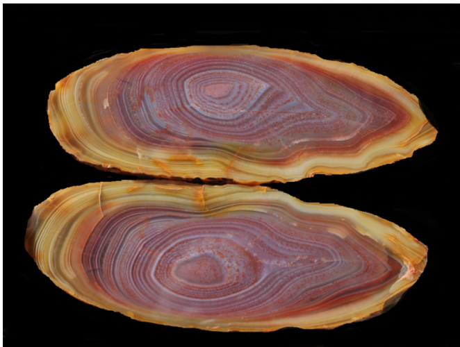
From the South Pacific near Indonesia. Rough nodule and polished halves.
