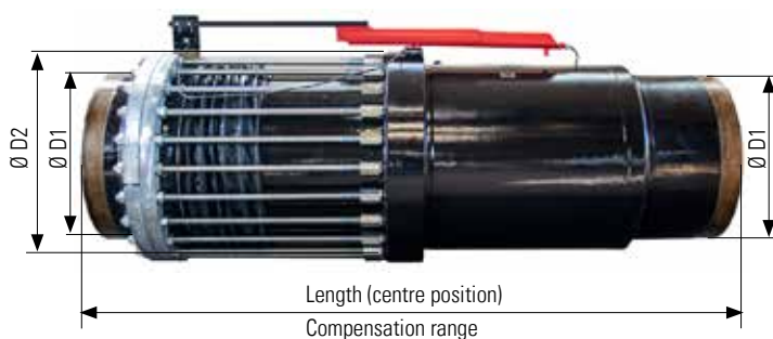
With pressure testing locking system (Compensator in centre position)
