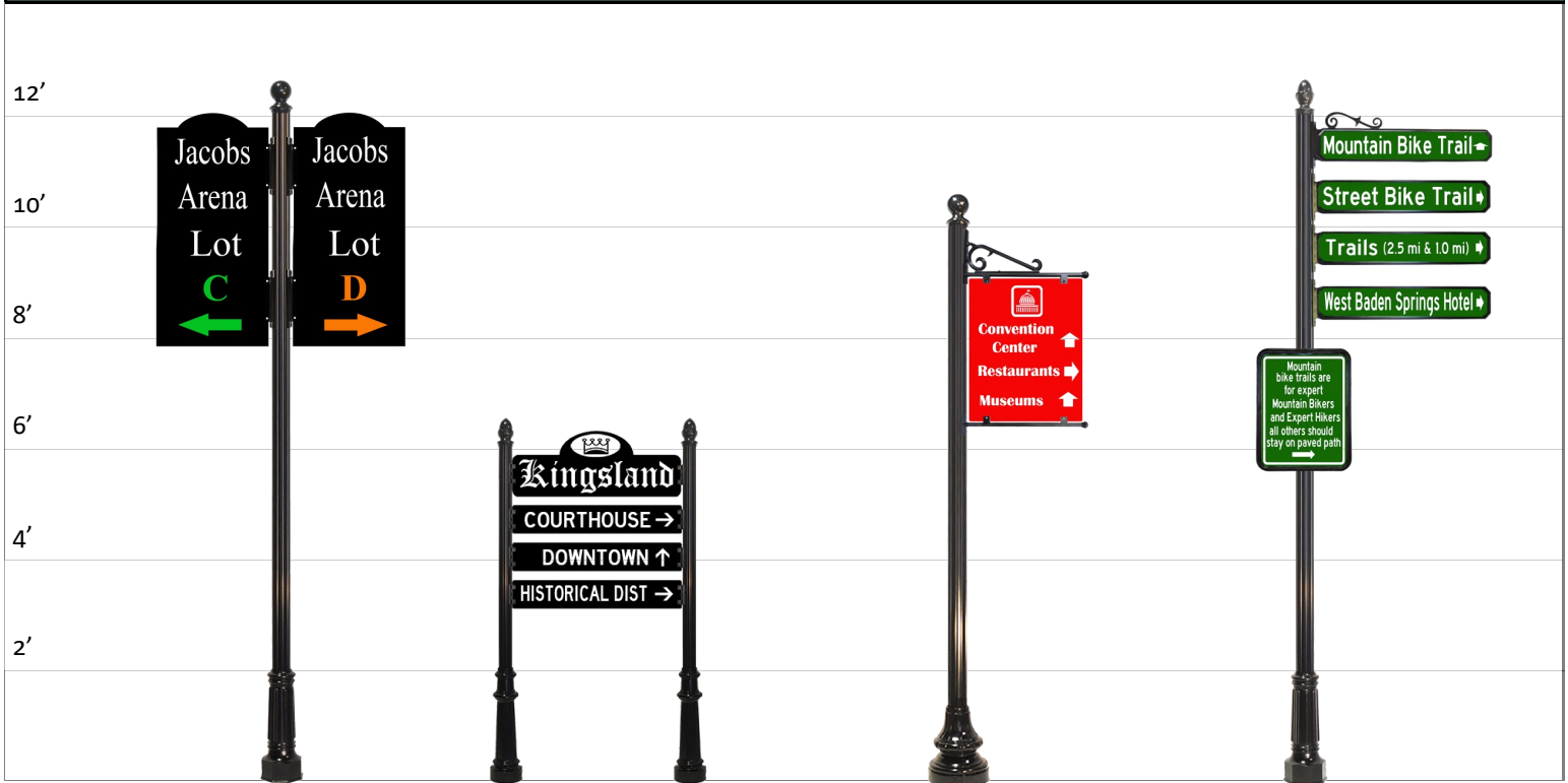
Wayfinding Sign A FL4X14 - 4"X14' Fluted Pole BALL4 - Ball Finial for 4" Pole BASE 42 - Two Piece Base for 4" Pole (4) BRK WF - Bracket for Flag Mounting large sign (2) Custom Wayfinding Sign
