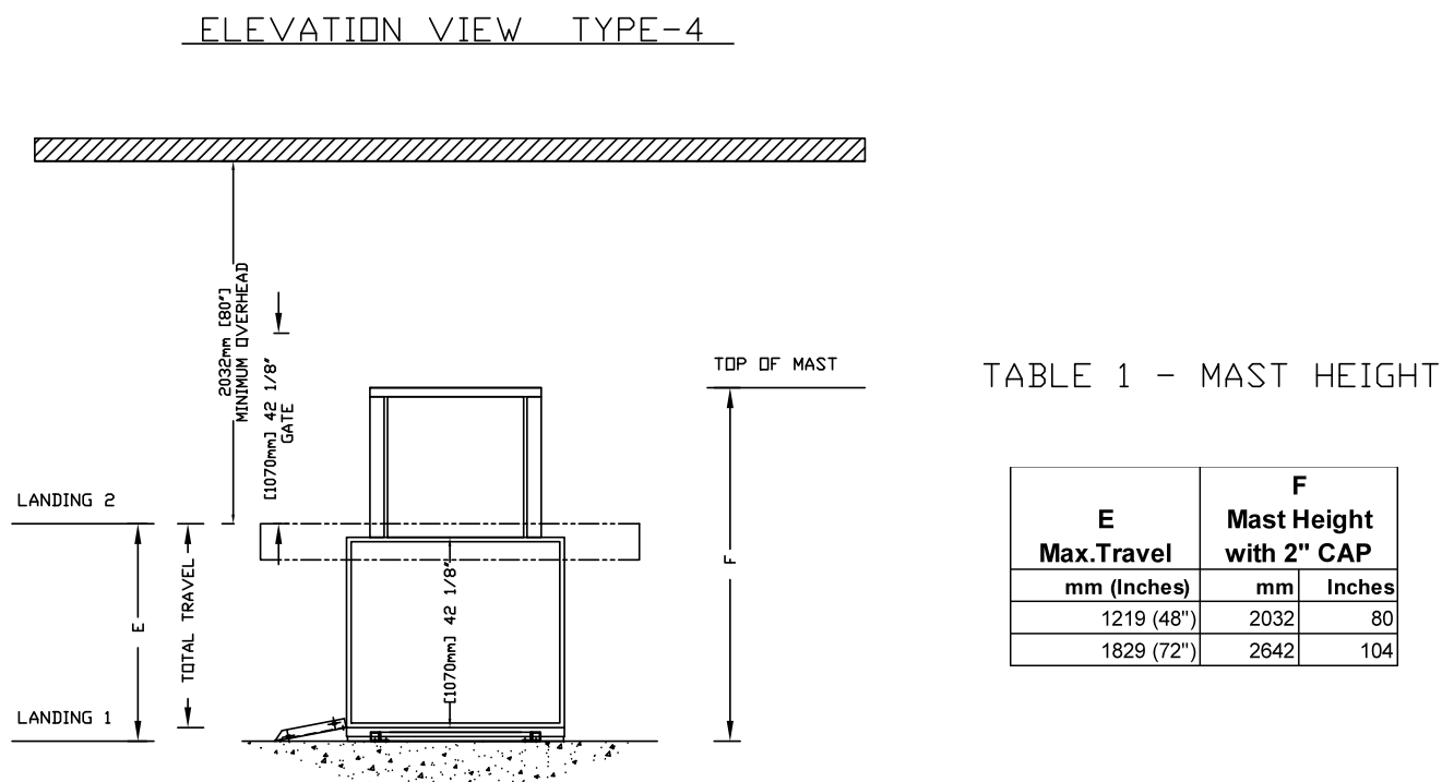
Figure 19: Elevation and plan view – type 4 without platform gate – 42" x 48", 42" x 54", 42" x 60"
