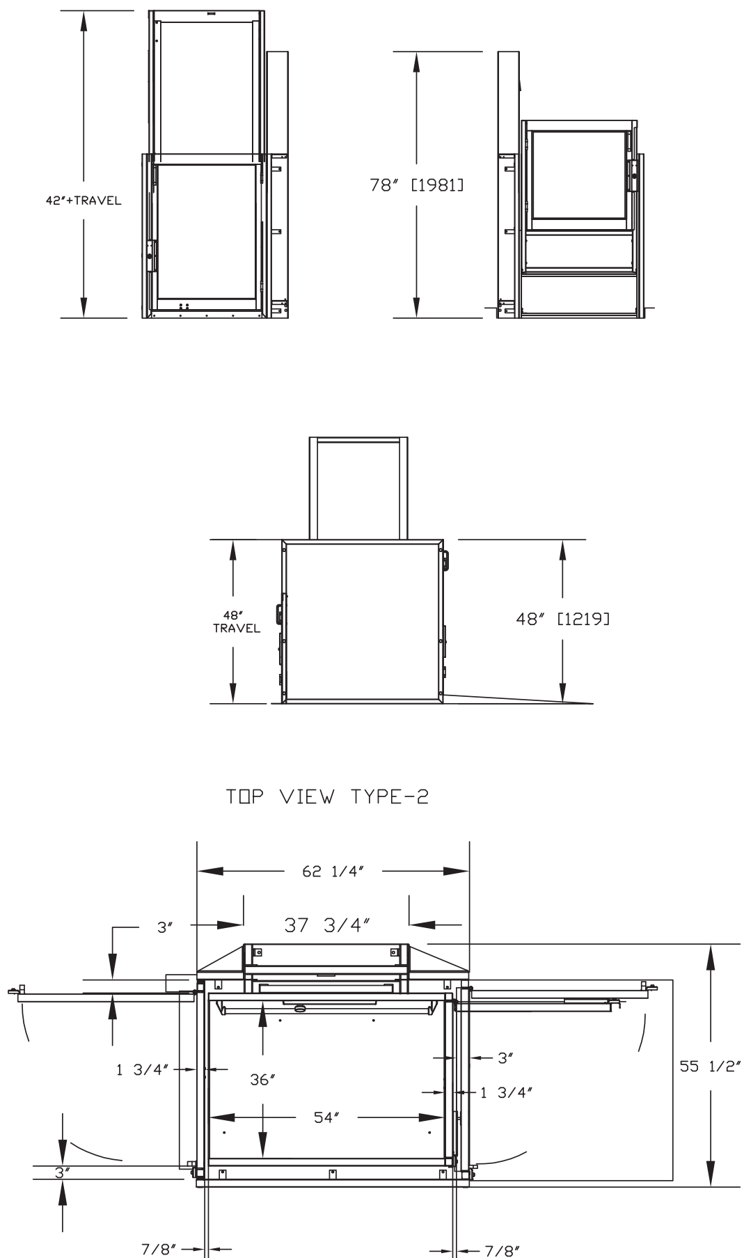
Figure 34: Elevation and plan view – type 2 with 3 gates (RH) – 36" x 54"
