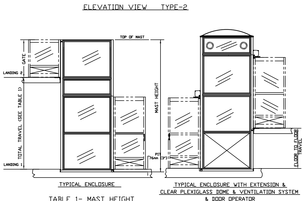
Figure 28: Elevation and plan view – type 2 enclosure – 36" x 48", 36" x 54", 36" x 60"
