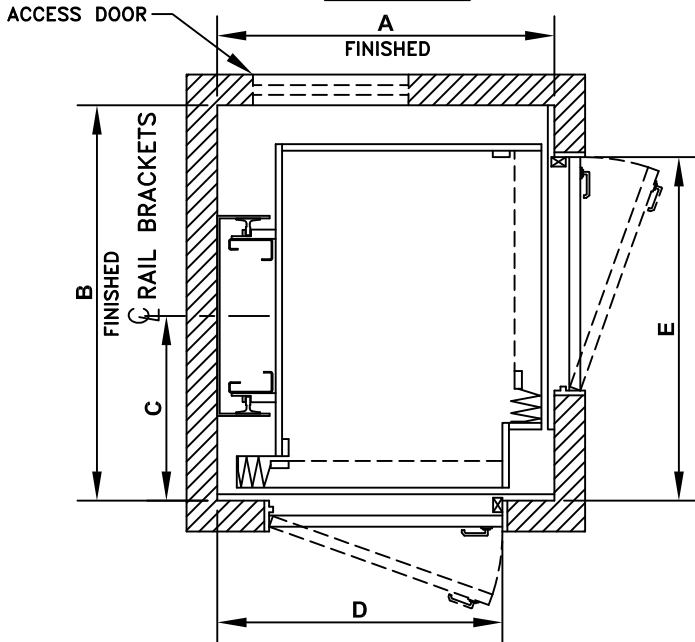
PLAN - E
