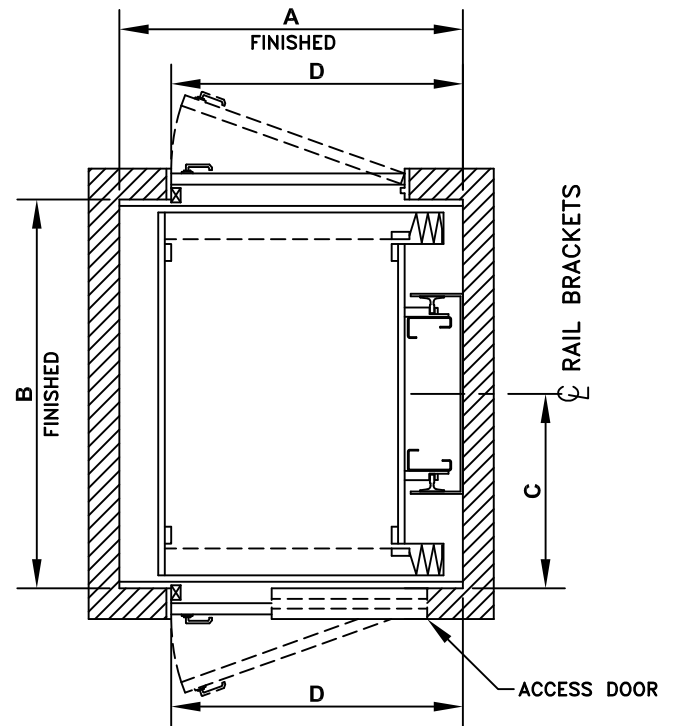
PLAN - H
