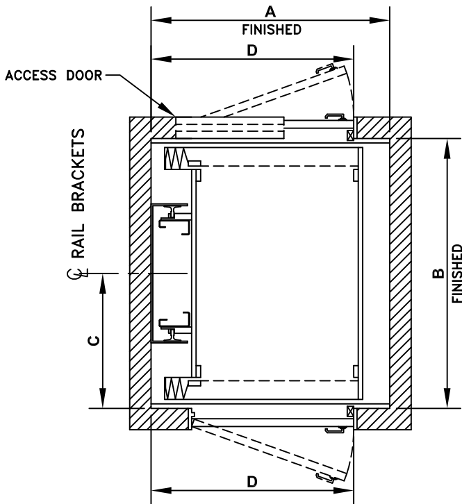
PLAN - G
