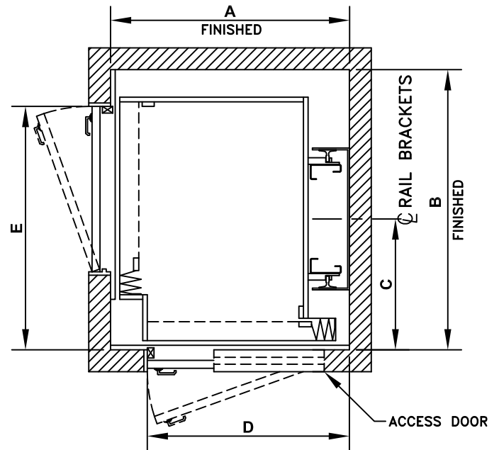
PLAN - F
