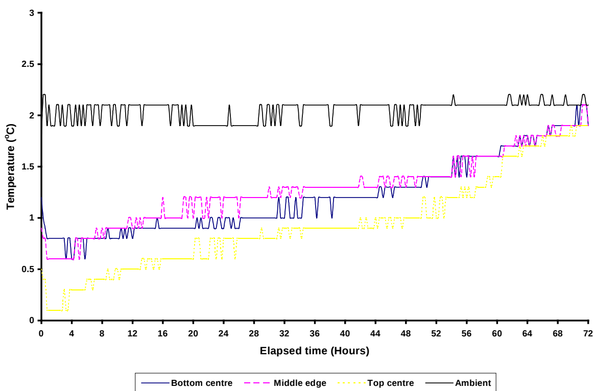
Figure 3.1. Average fillet temperature in the EPS box held in a constant ambient temperature of 2°C for 72hours (gel-ice cooling of fillets).
