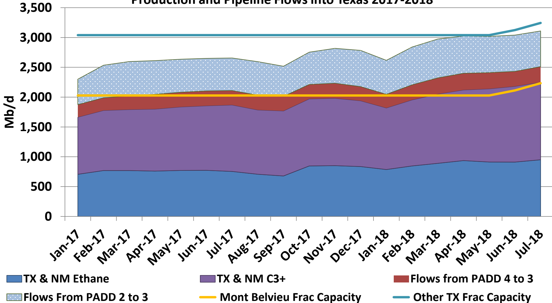
Texas Fractionator Capacity vs. TX & NM Raw Mix NGL Production and Pipeline Flows into Texas 2017-2018
