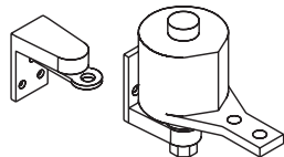
Mortised Box and Reversed Brackets
