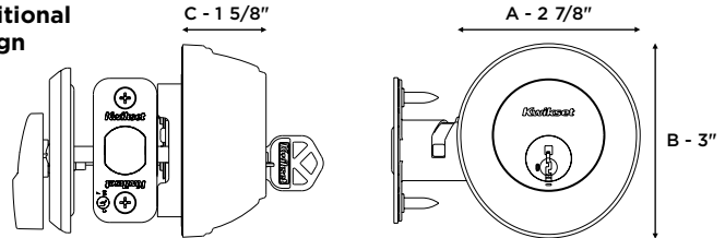
817 UL Key Control Deadbolt Deadbolt operated by key outside and thumb turn inside.
